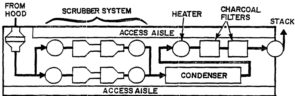
OFF-GAS TRAILER
