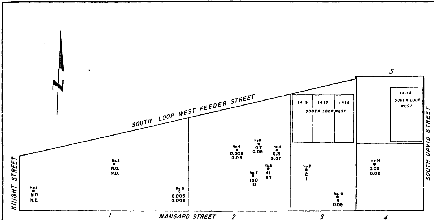
FIGURE I-5 TCE VALUES IN SHALLOW BOREHOLE SOIL SAMPLES (PPM)
