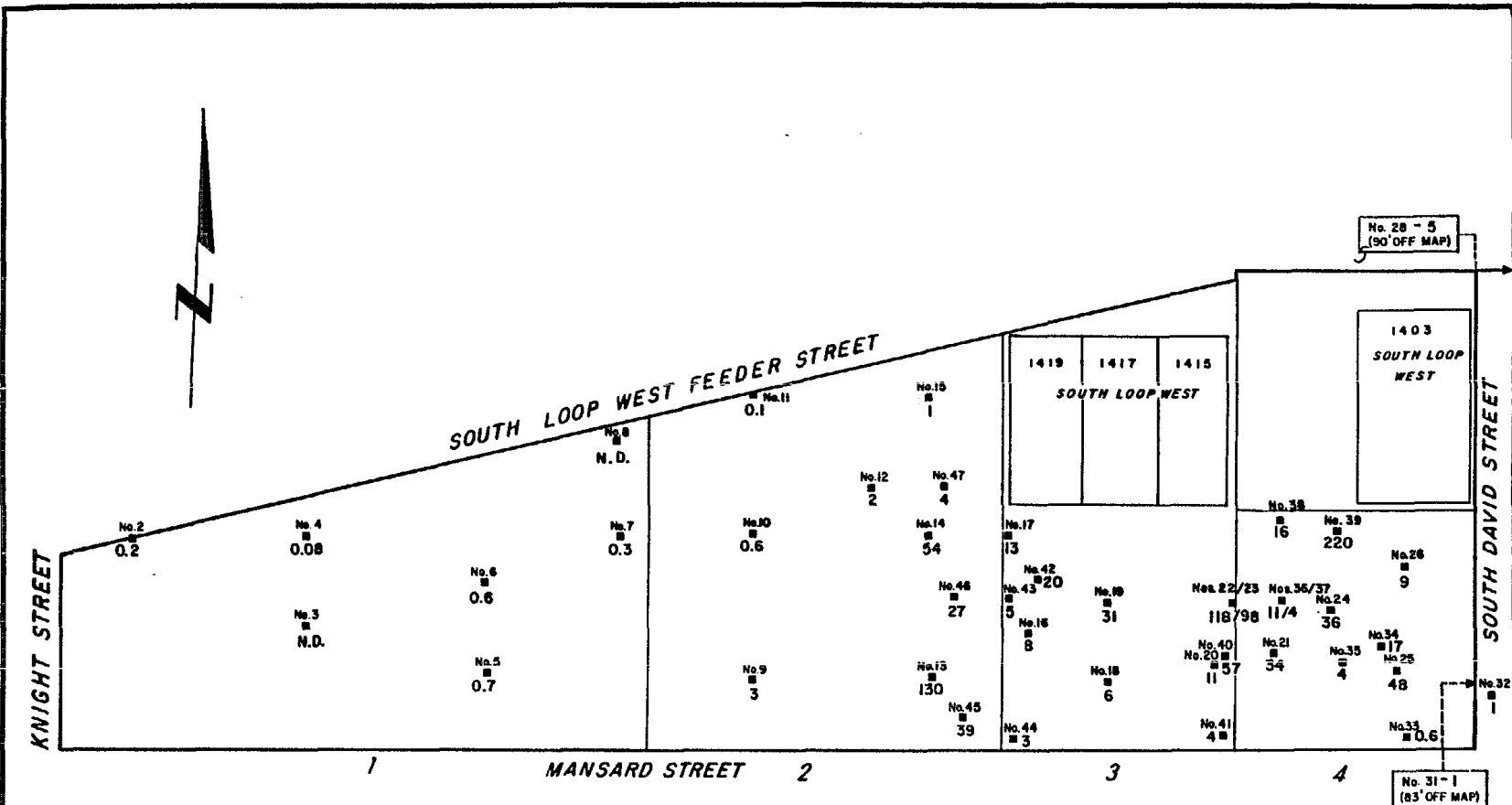
FIGURE I-2 PCB VALUES IN SURFACE SOIL SAMPLES (PPM)
